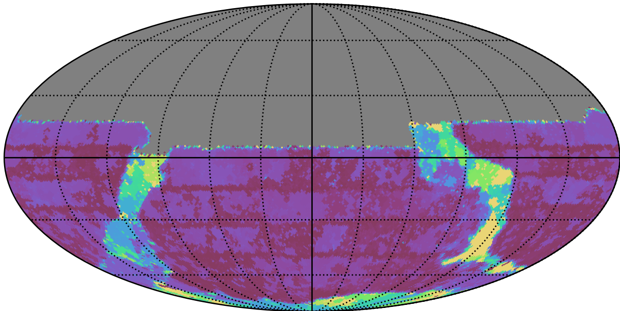
ddf_loaded_fl1_v3.4_10yrs All sky u band: Max Inter-Night Gap
