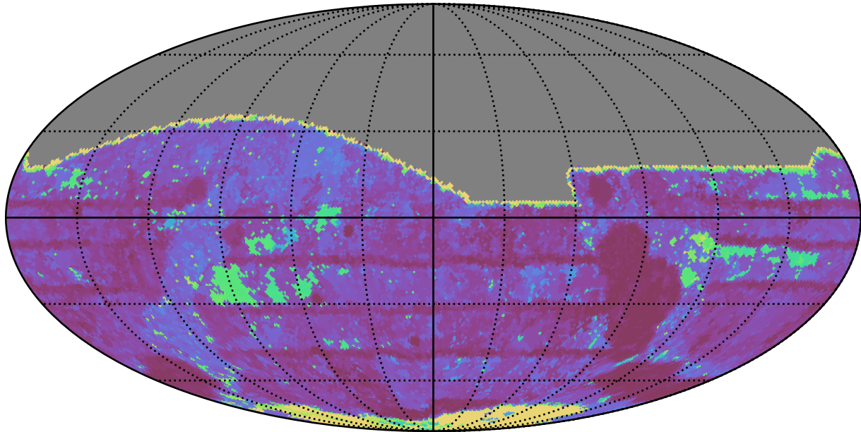
ddf_loaded_fl1_v3.4_10yrs All sky r band: Max Inter-Night Gap
