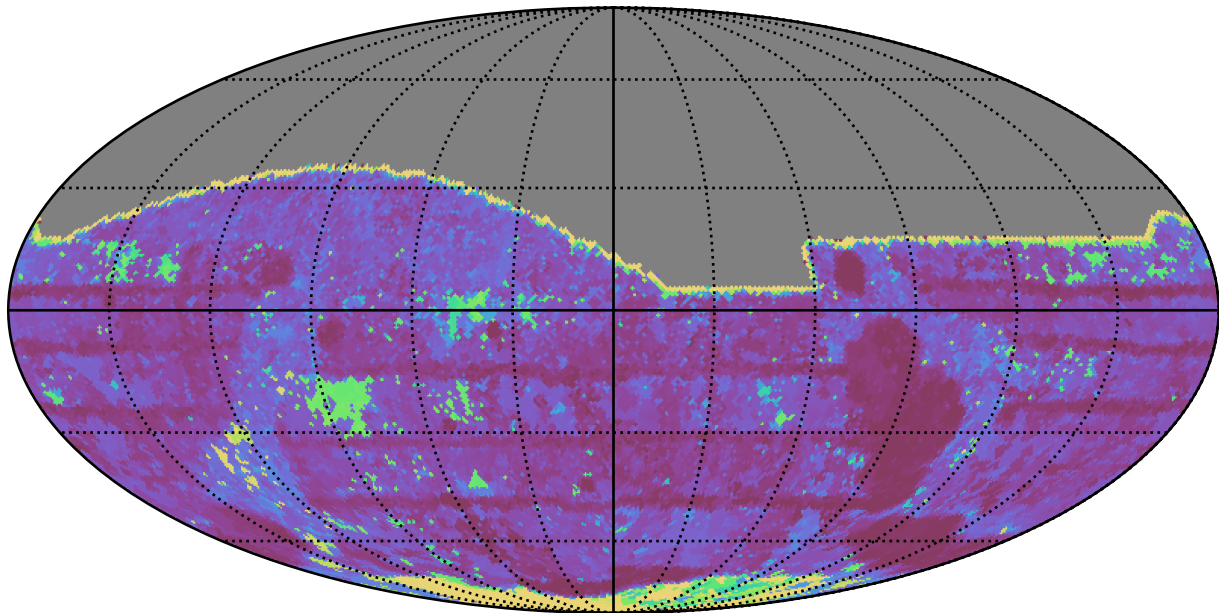
ddf_loaded_fl1_v3.4_10yrs All sky i band: Max Inter-Night Gap
