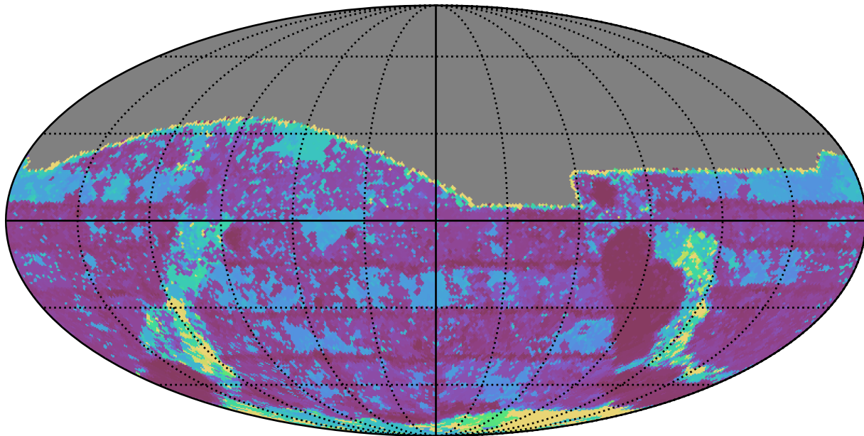
ddf_loaded_fl1_v3.4_10yrs All sky g band: Max Inter-Night Gap
