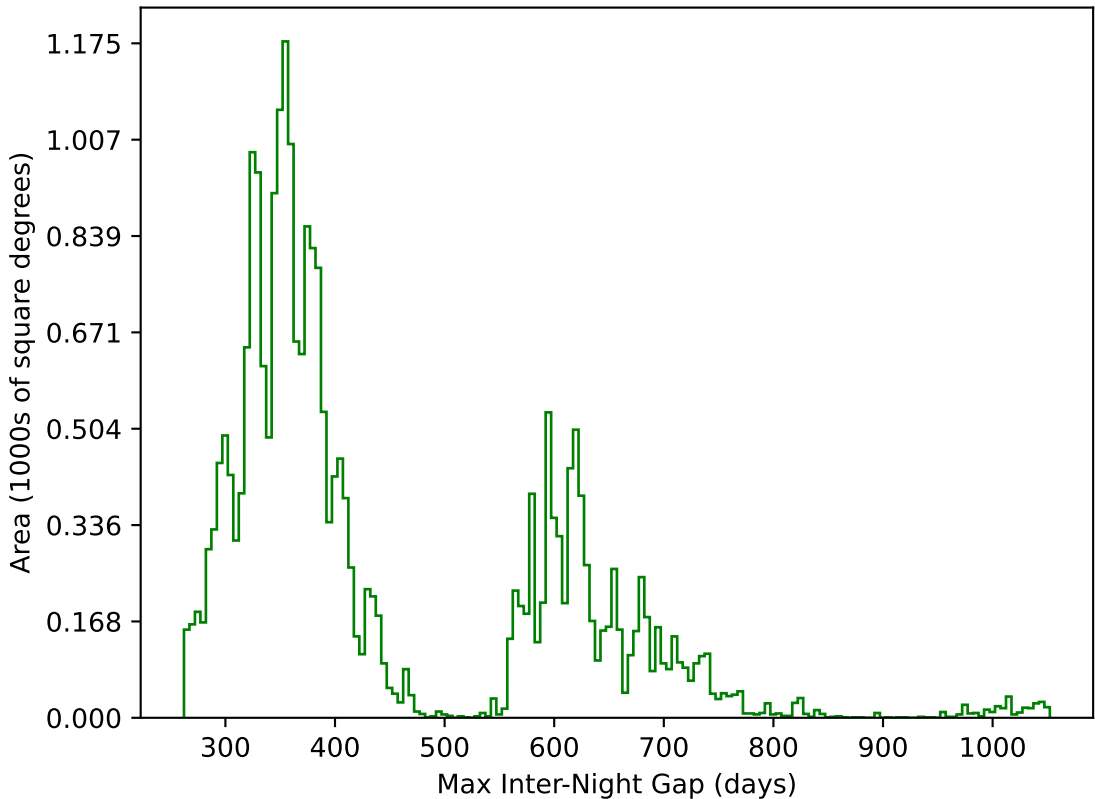
ddf_loaded_fl1_v3.4_10yrs All sky g band: Max Inter-Night Gap
