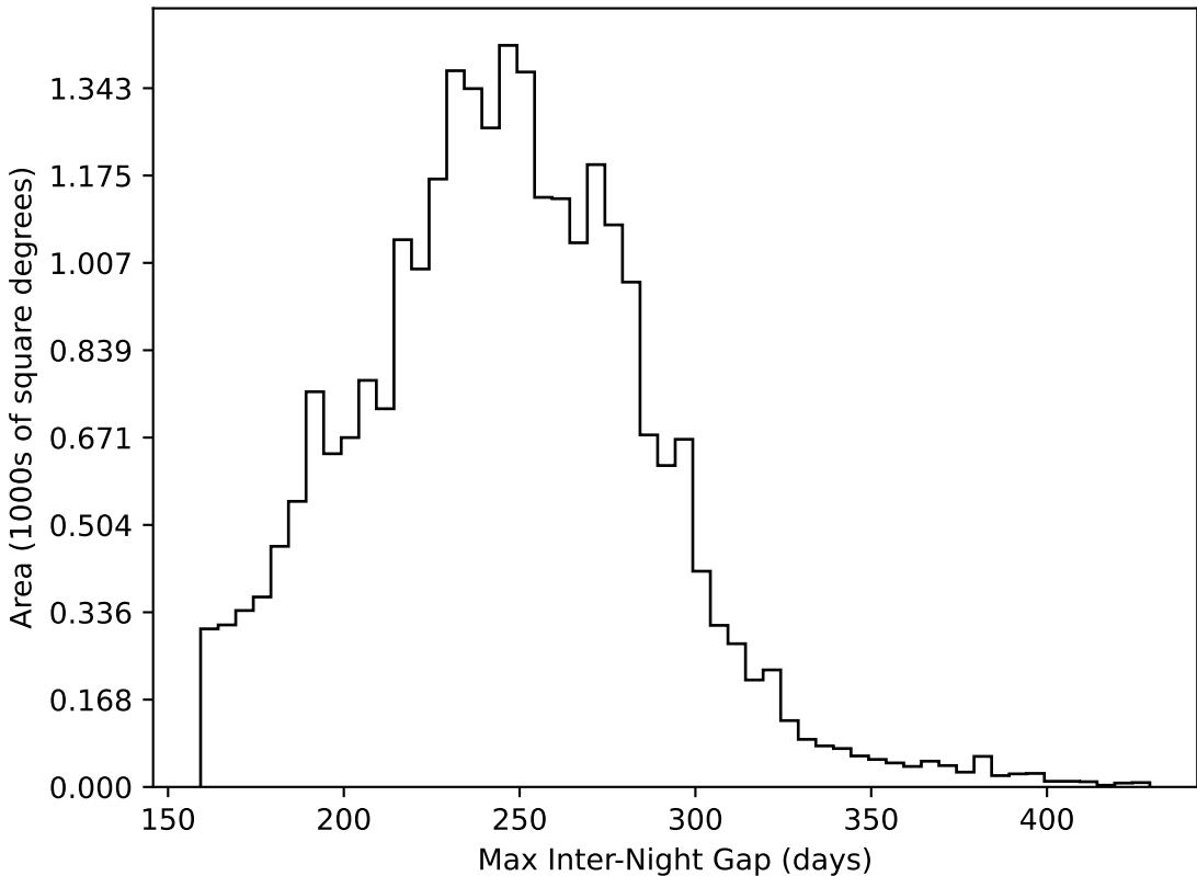
ddf_loaded_fl1_v3.4_10yrs All sky all bands: Max Inter-Night Gap
