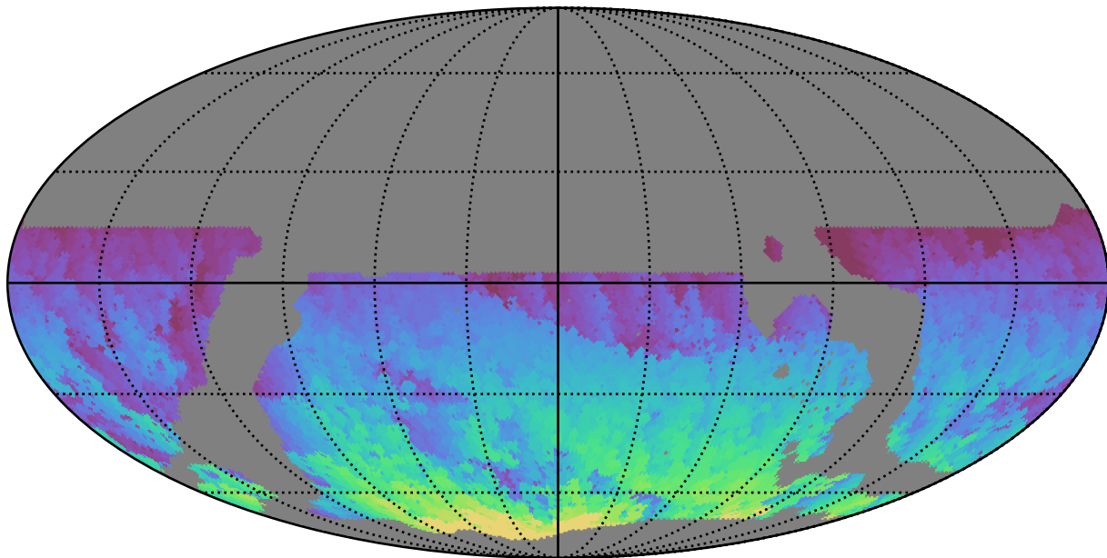
ddf_loaded_fl1_v3.4_10yrs WFD z band: Max HA
