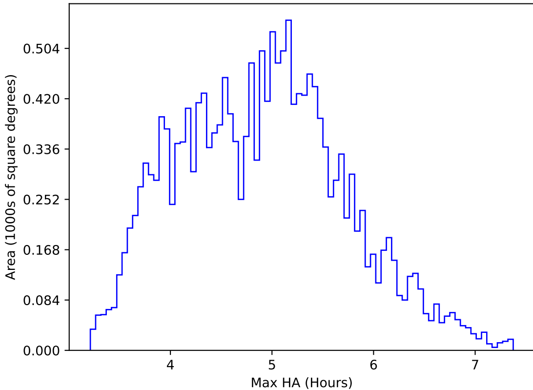
ddf_loaded_fl1_v3.4_10yrs WFD z band: Max HA
