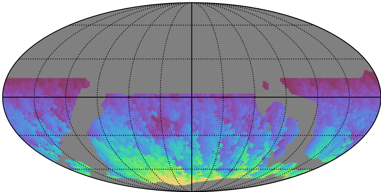
ddf_loaded_fl1_v3.4_10yrs WFD y band: Max HA
