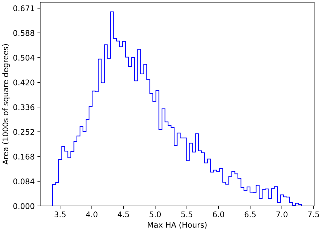
ddf_loaded_fl1_v3.4_10yrs WFD y band: Max HA
