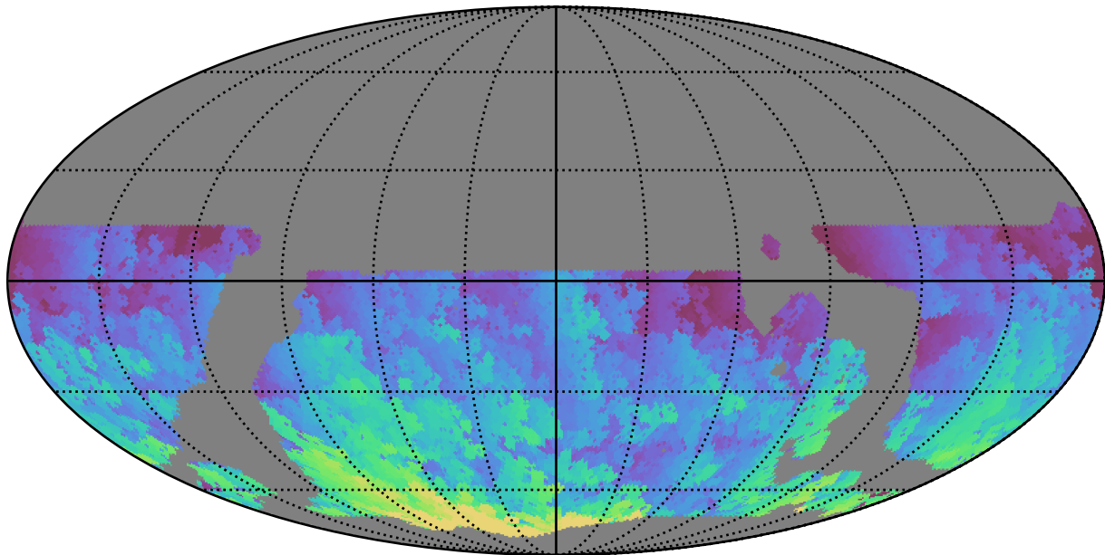
ddf_loaded_fl1_v3.4_10yrs WFD u band: Max HA
