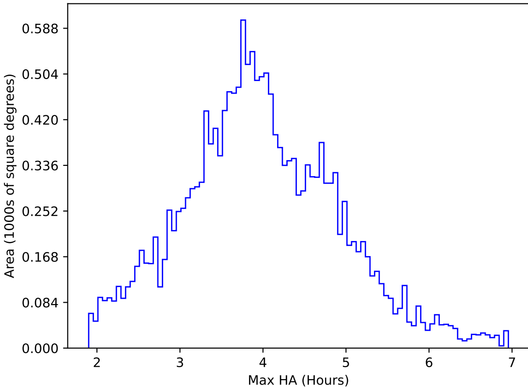
ddf_loaded_fl1_v3.4_10yrs WFD u band: Max HA
