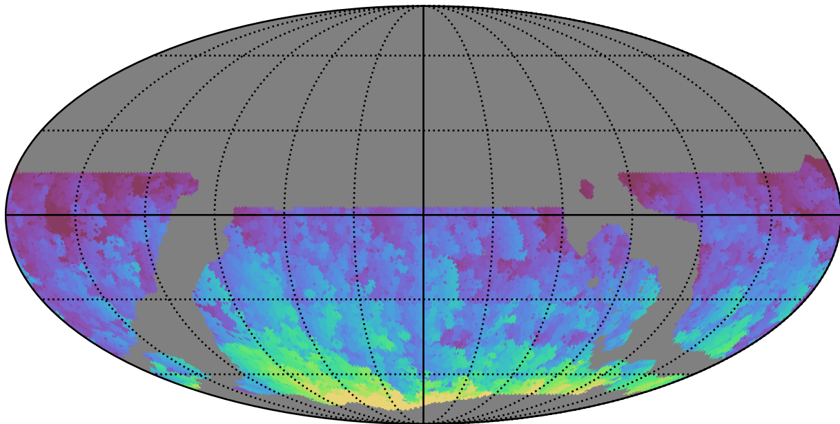
ddf_loaded_fl1_v3.4_10yrs WFD r band: Max HA
