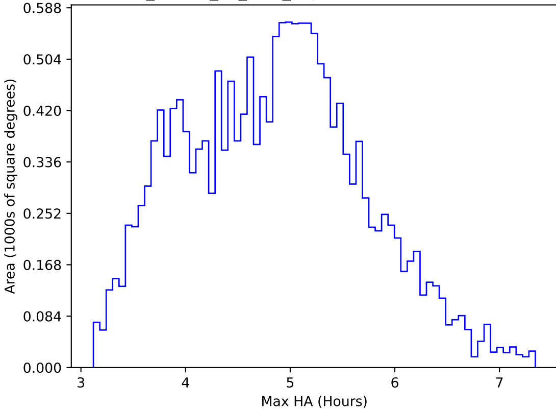
ddf_loaded_fl1_v3.4_10yrs WFD i band: Max HA
