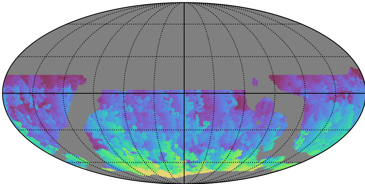
ddf_loaded_fl1_v3.4_10yrs WFD g band: Max HA
