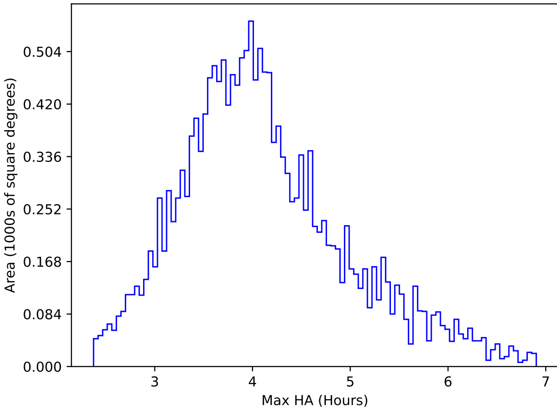
ddf_loaded_fl1_v3.4_10yrs WFD g band: Max HA
