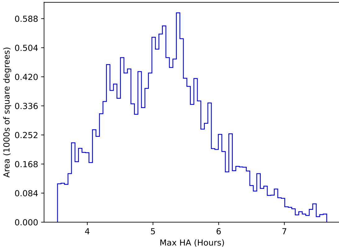
ddf_loaded_fl1_v3.4_10yrs WFD all bands: Max HA
