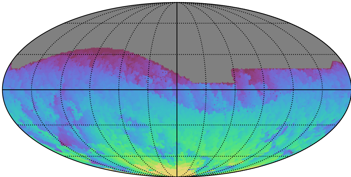
ddf_loaded_fl1_v3.4_10yrs All sky z band: Max HA
