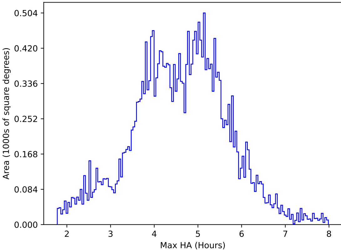
ddf_loaded_fl1_v3.4_10yrs All sky z band: Max HA
