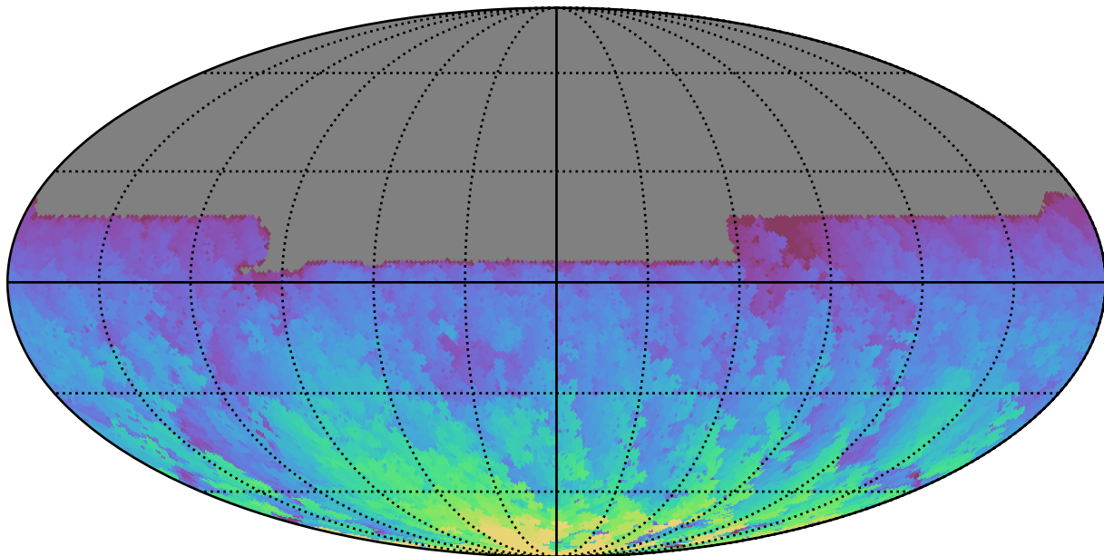
ddf_loaded_fl1_v3.4_10yrs All sky y band: Max HA
