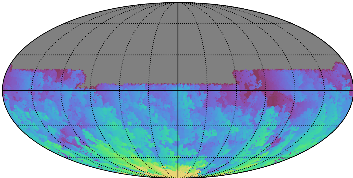
ddf_loaded_fl1_v3.4_10yrs All sky u band: Max HA
