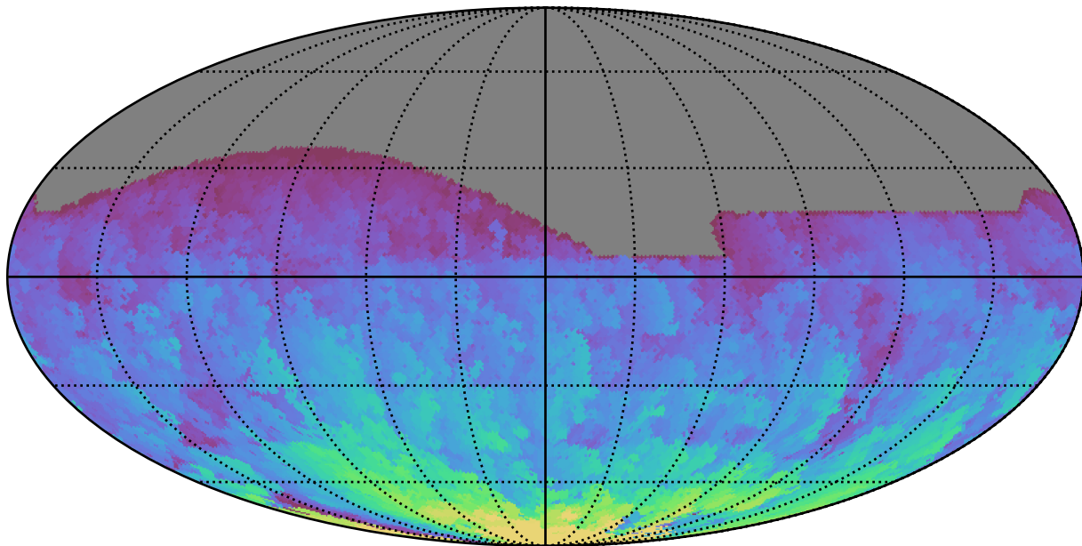
ddf_loaded_fl1_v3.4_10yrs All sky r band: Max HA
