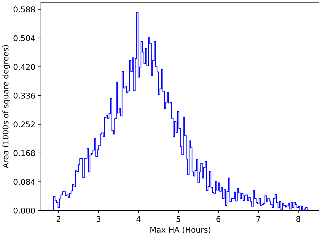
ddf_loaded_fl1_v3.4_10yrs All sky r band: Max HA
