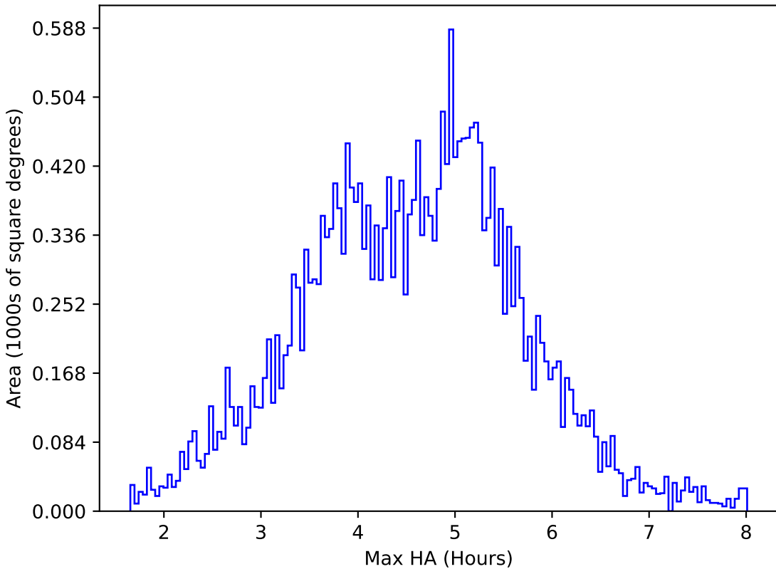
ddf_loaded_fl1_v3.4_10yrs All sky i band: Max HA
