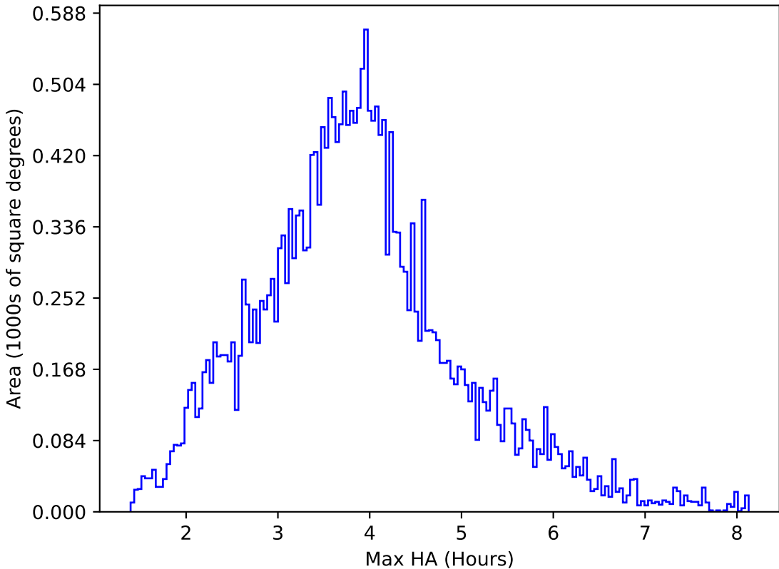
ddf_loaded_fl1_v3.4_10yrs All sky g band: Max HA
