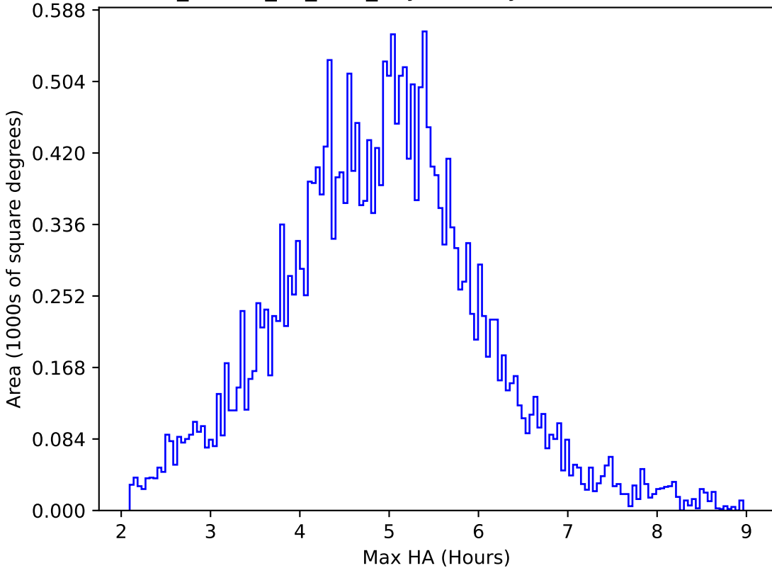
ddf_loaded_fl1_v3.4_10yrs All sky all bands: Max HA
