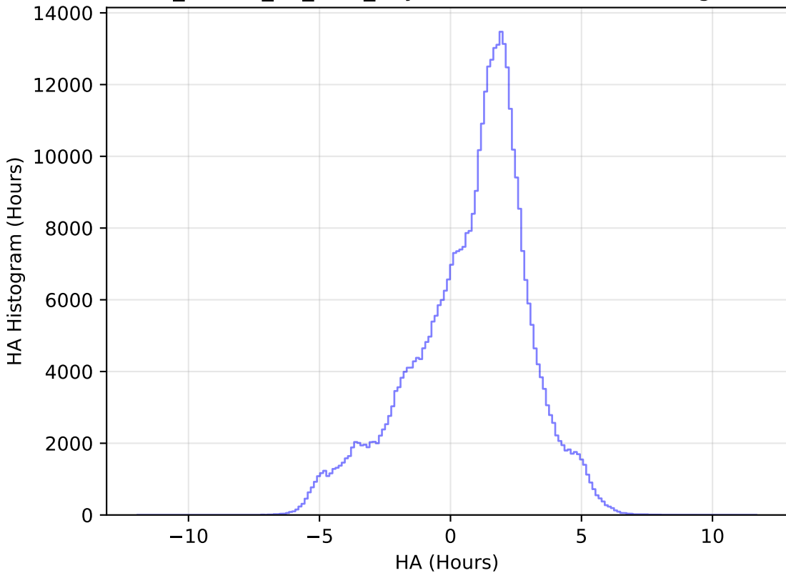
ddf_loaded_fl1_v3.4_10yrs WFD z band: HA Histogram
