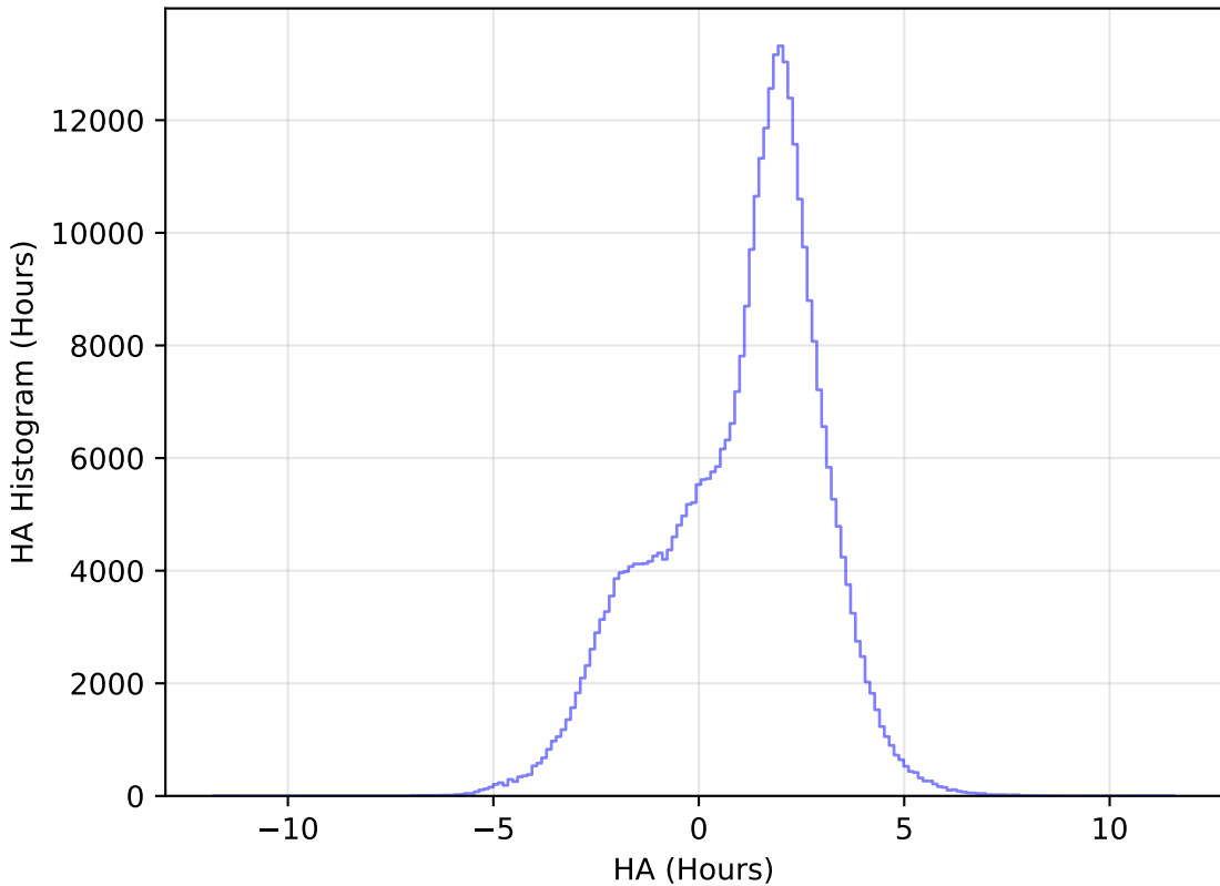
ddf_loaded_fl1_v3.4_10yrs WFD y band: HA Histogram
