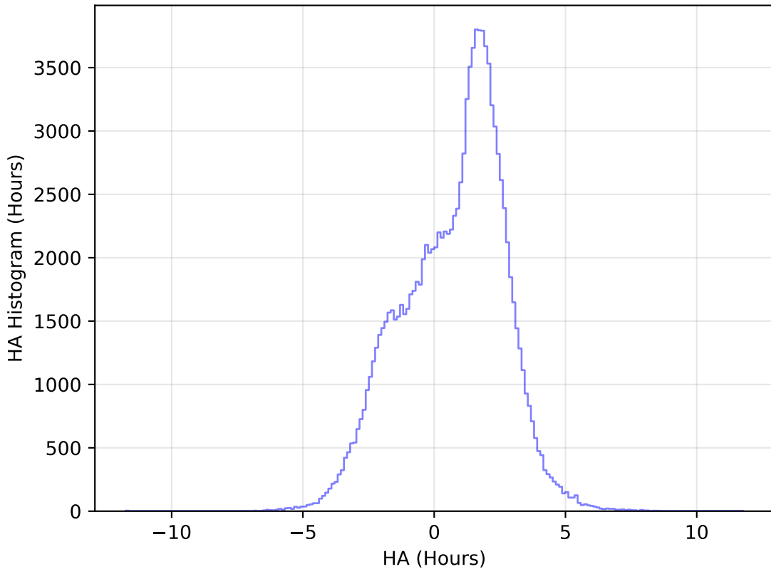
ddf_loaded_fl1_v3.4_10yrs WFD u band: HA Histogram
