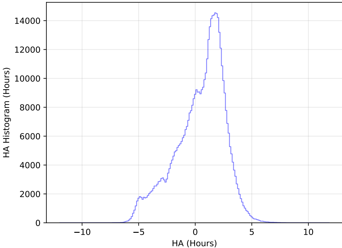
ddf_loaded_fl1_v3.4_10yrs WFD r band: HA Histogram
