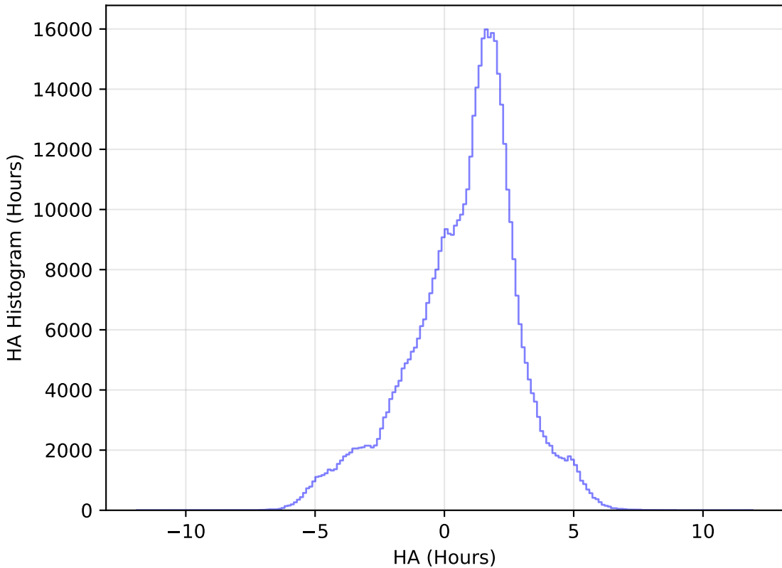
ddf_loaded_fl1_v3.4_10yrs WFD i band: HA Histogram
