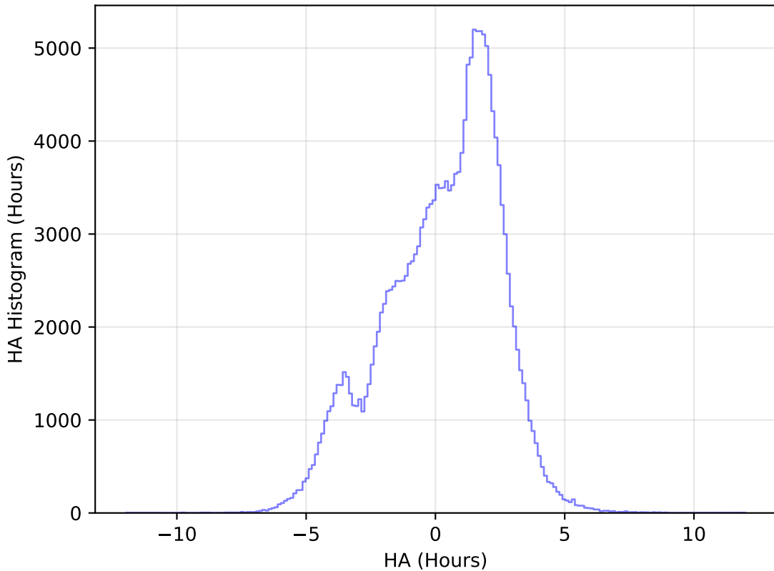
ddf_loaded_fl1_v3.4_10yrs WFD g band: HA Histogram
