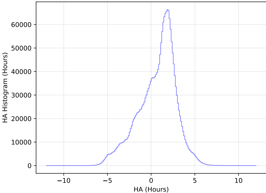
ddf_loaded_fl1_v3.4_10yrs WFD all bands: HA Histogram
