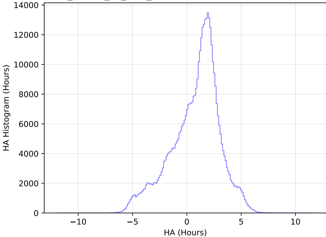
ddf_loaded_fl1_v3.4_10yrs All sky z band: HA Histogram
