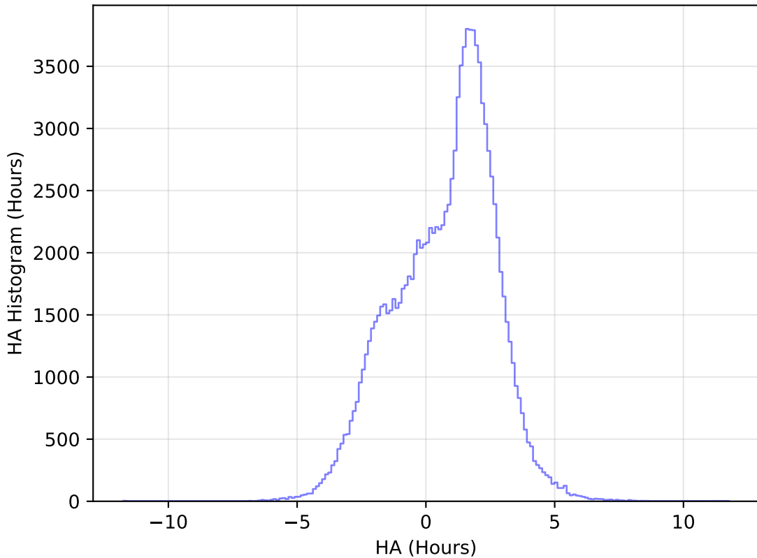
ddf_loaded_fl1_v3.4_10yrs All sky u band: HA Histogram
