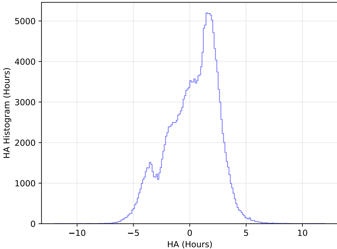
ddf_loaded_fl1_v3.4_10yrs All sky g band: HA Histogram
