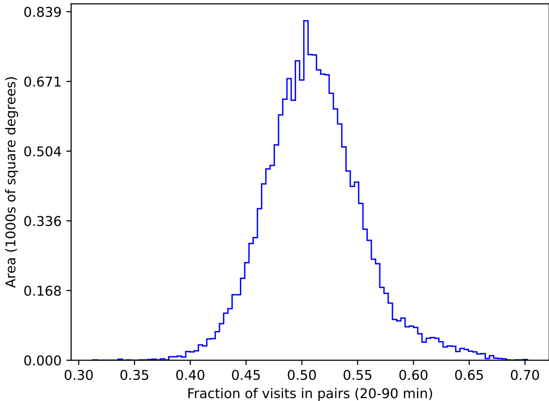
ddf_loaded_fl1_v3.4_10yrs gri WFD: Fraction of visits in pairs (20-90 min)
