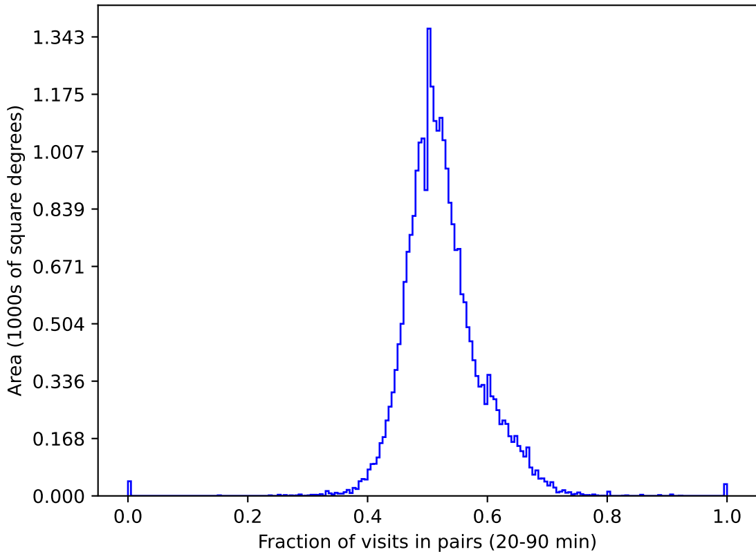
ddf_loaded_fl1_v3.4_10yrs gri All sky: Fraction of visits in pairs (20-90 min)
