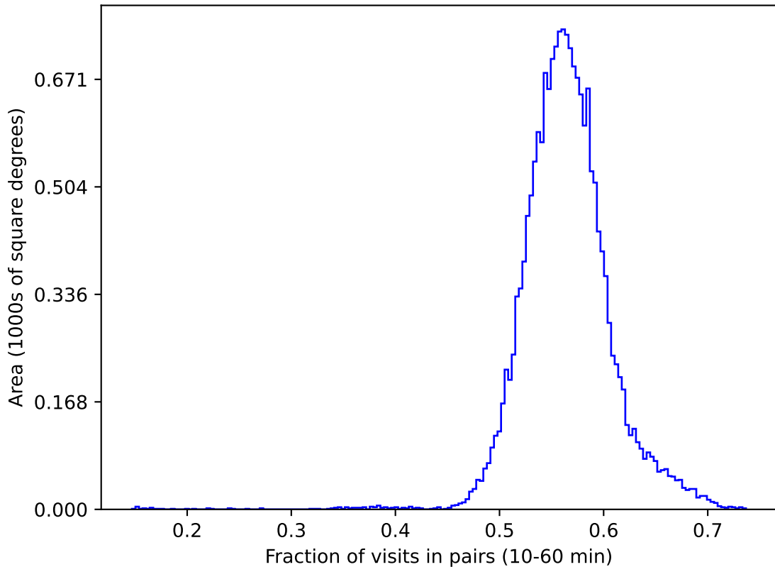
ddf_loaded_fl1_v3.4_10yrs gri WFD: Fraction of visits in pairs (10-60 min)
