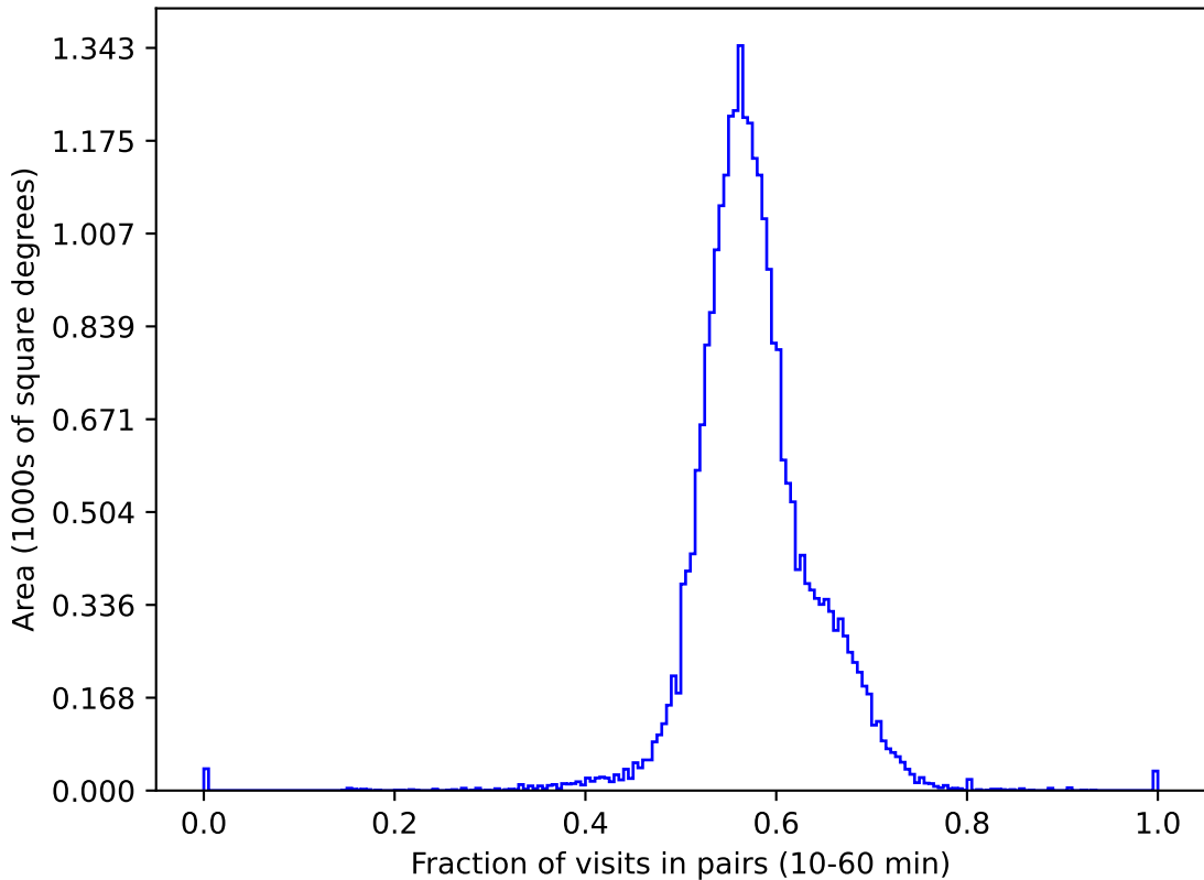
ddf_loaded_fl1_v3.4_10yrs gri All sky: Fraction of visits in pairs (10-60 min)
