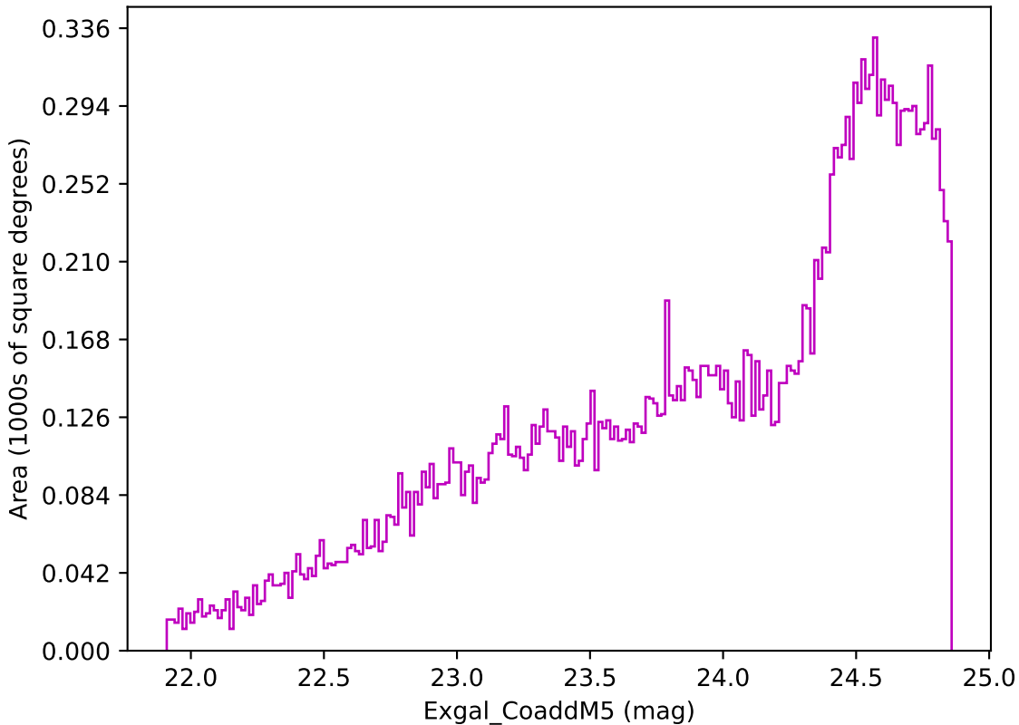
ddf_loaded_fl1_v3.4_10yrs Yr 3-4 z band: Exgal_CoaddM5
