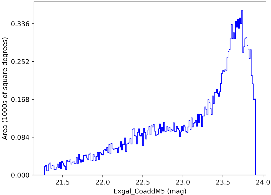
ddf_loaded_fl1_v3.4_10yrs Yr 3-4 y band: Exgal_CoaddM5
