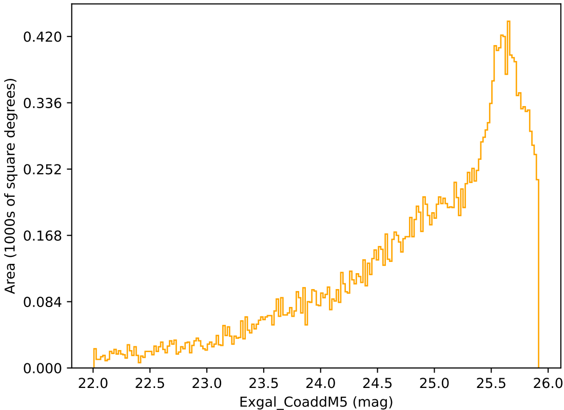
ddf_loaded_fl1_v3.4_10yrs Yr 3-4 r band: Exgal_CoaddM5
