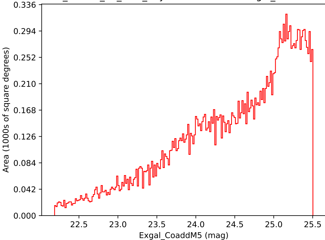
ddf_loaded_fl1_v3.4_10yrs Yr 3-4 i band: Exgal_CoaddM5
