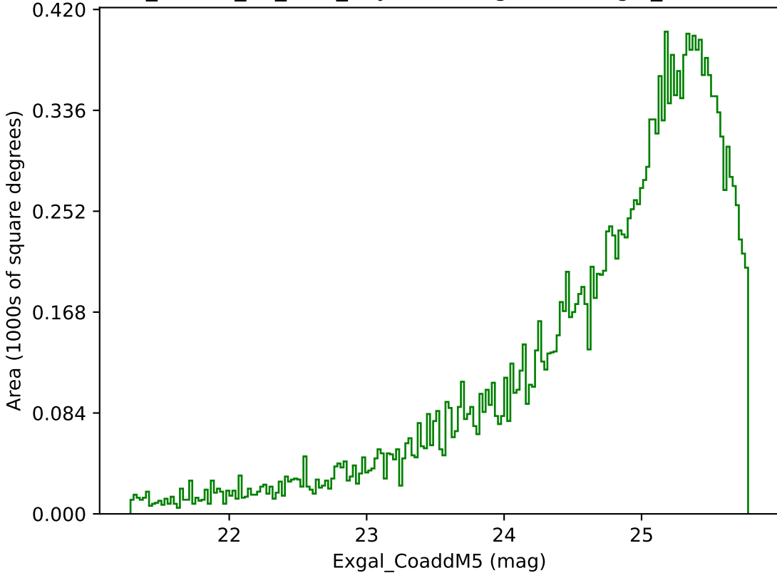
ddf_loaded_fl1_v3.4_10yrs Yr 3-4 g band: Exgal_CoaddM5
