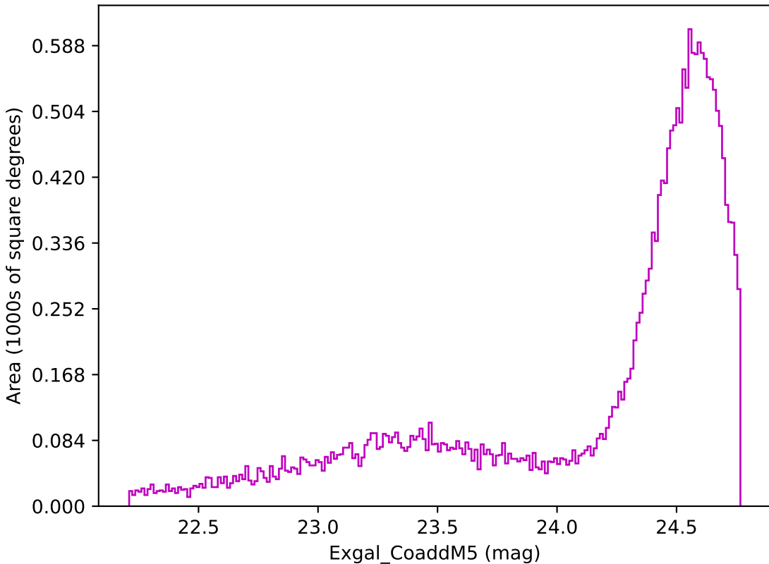
ddf_loaded_fl1_v3.4_10yrs Yr 1 z band: Exgal_CoaddM5
