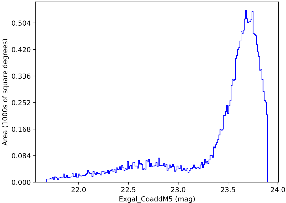
ddf_loaded_fl1_v3.4_10yrs Yr 1 y band: Exgal_CoaddM5
