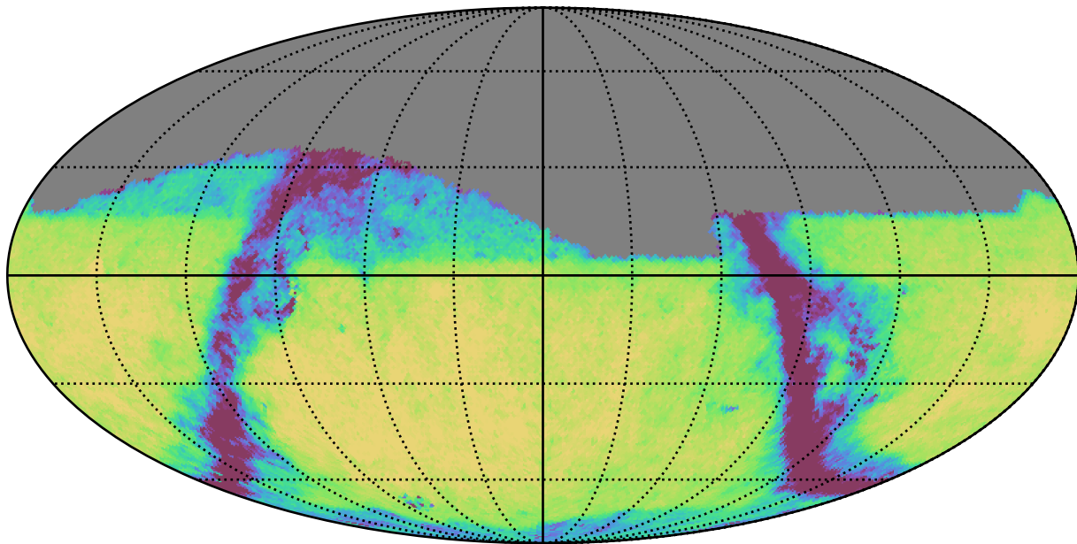
ddf_loaded_fl1_v3.4_10yrs Yr 1 r band: Exgal_CoaddM5
