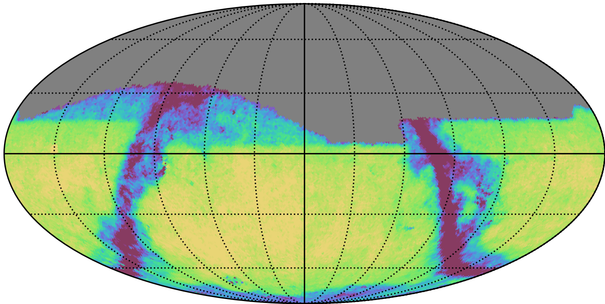
ddf_loaded_fl1_v3.4_10yrs Yr 1 i band: Exgal_CoaddM5
