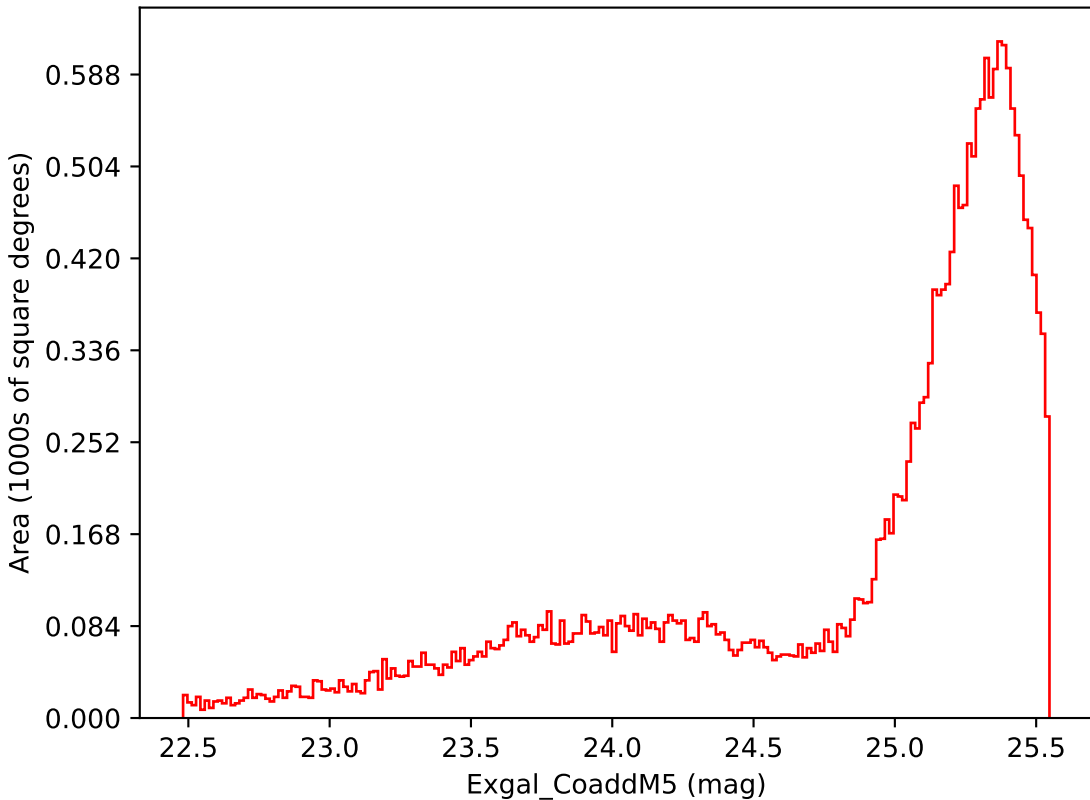
ddf_loaded_fl1_v3.4_10yrs Yr 1 i band: Exgal_CoaddM5
